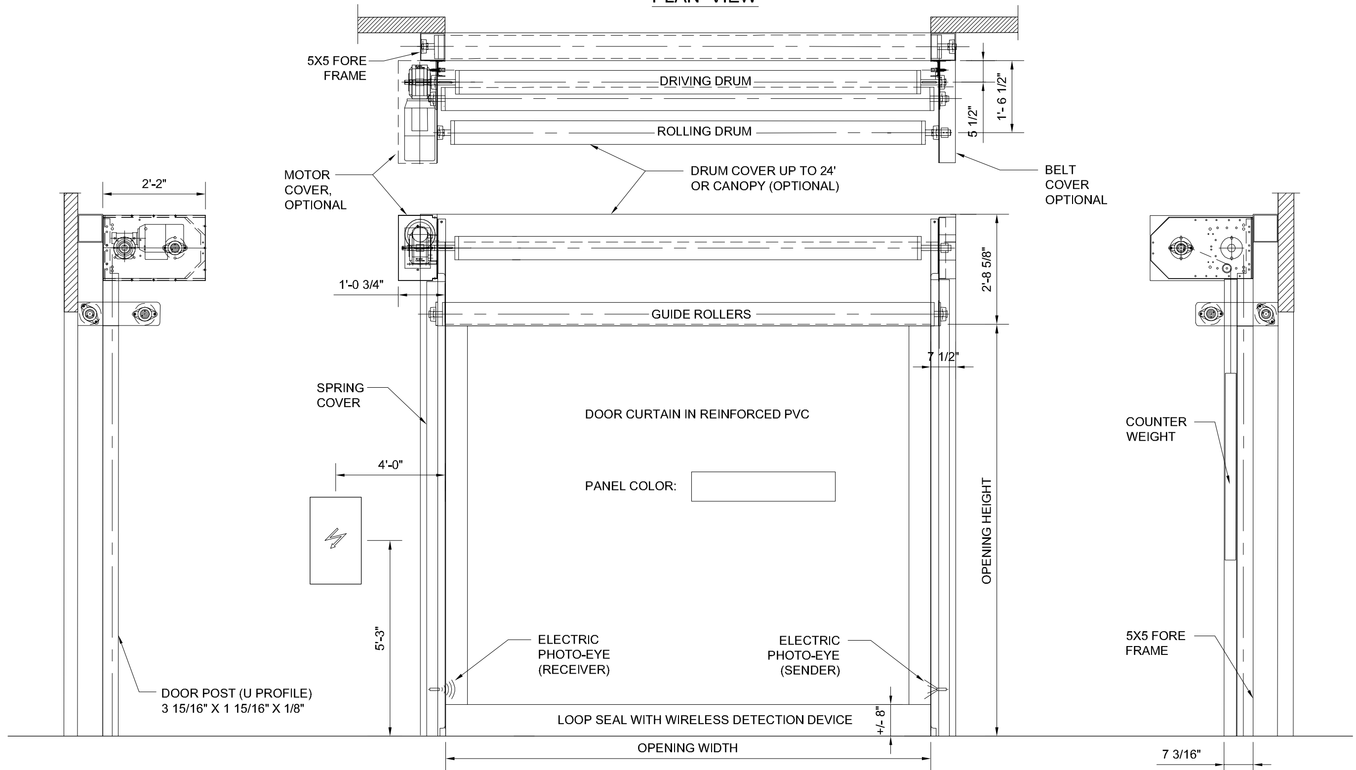
ELEVATION VIEW - LEFT
